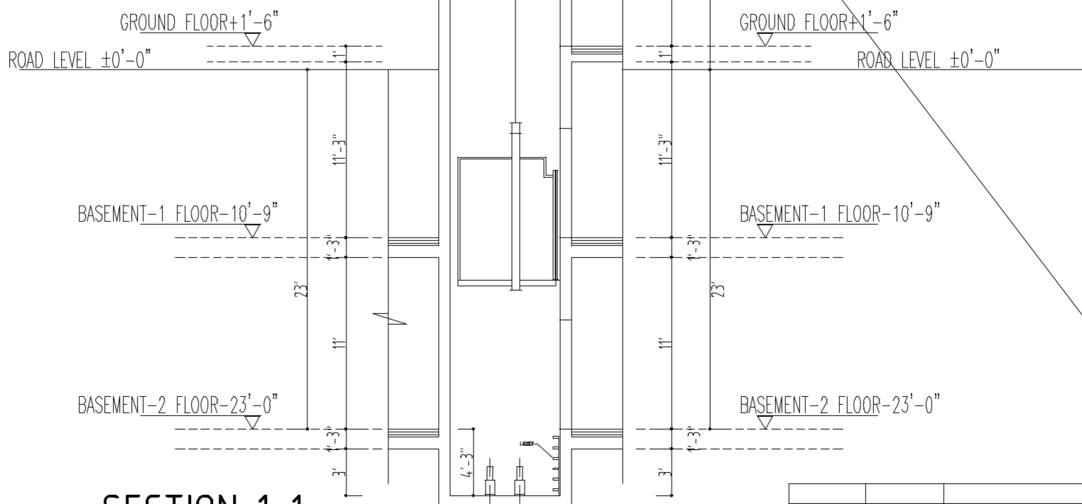
SECTION 1-1
